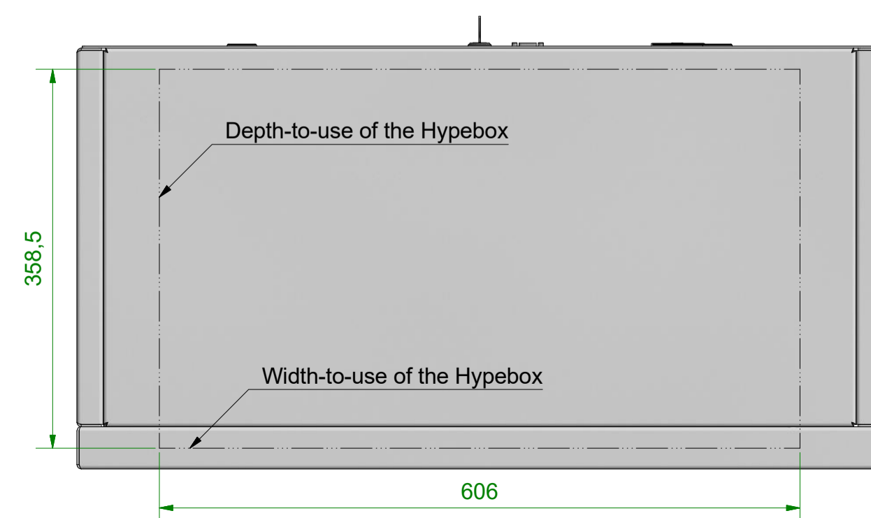
Top View 1:5
