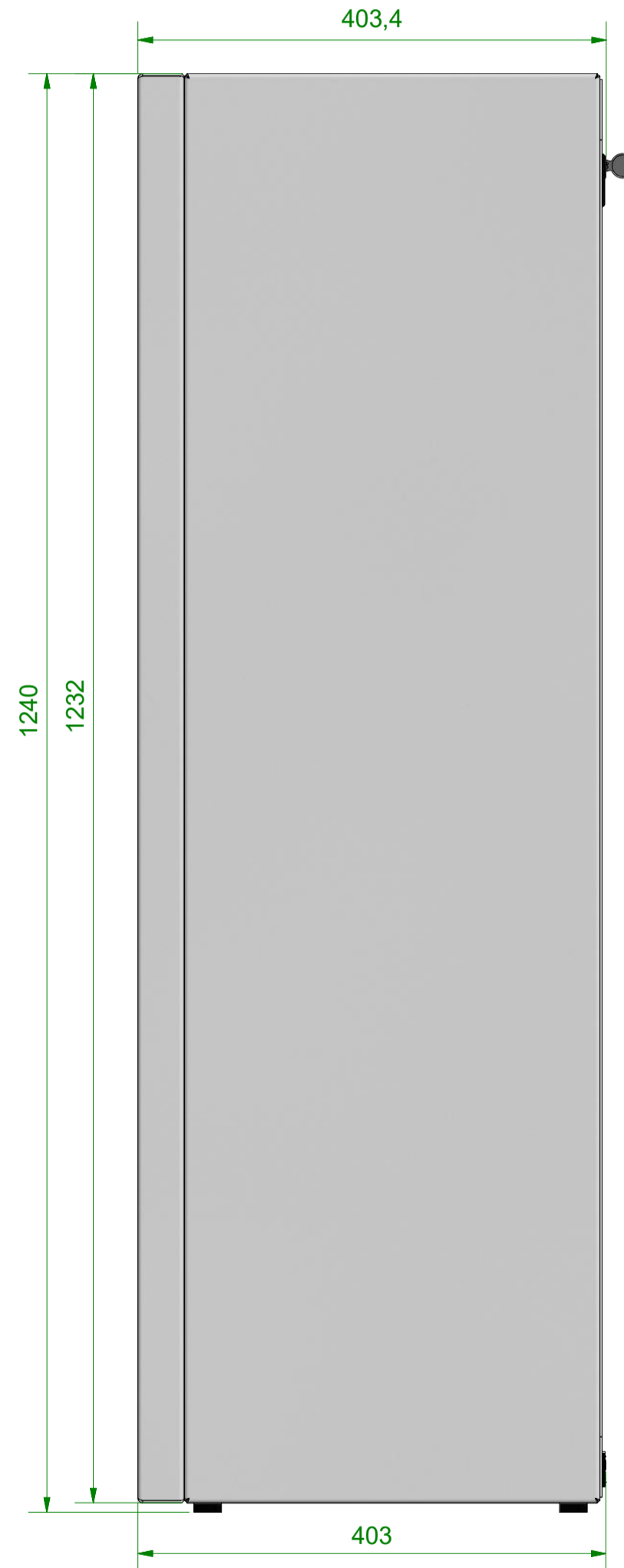
Righthand View 1:5
