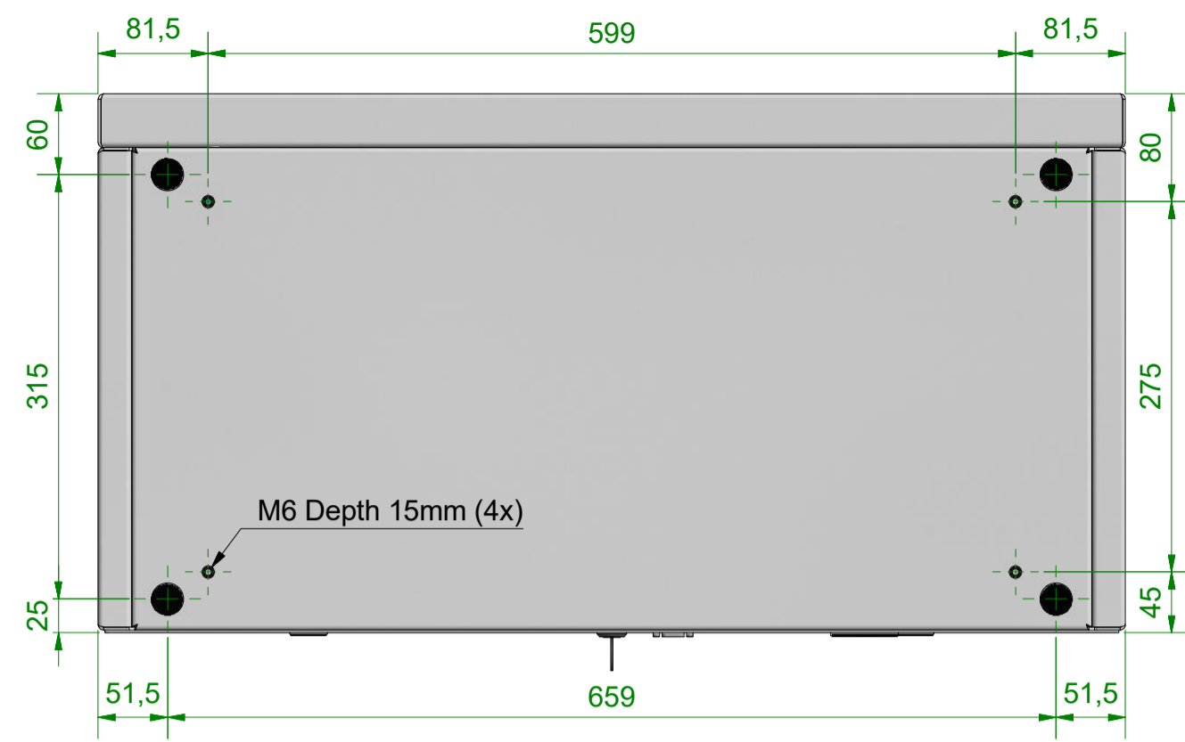
Bottom View 1:5
