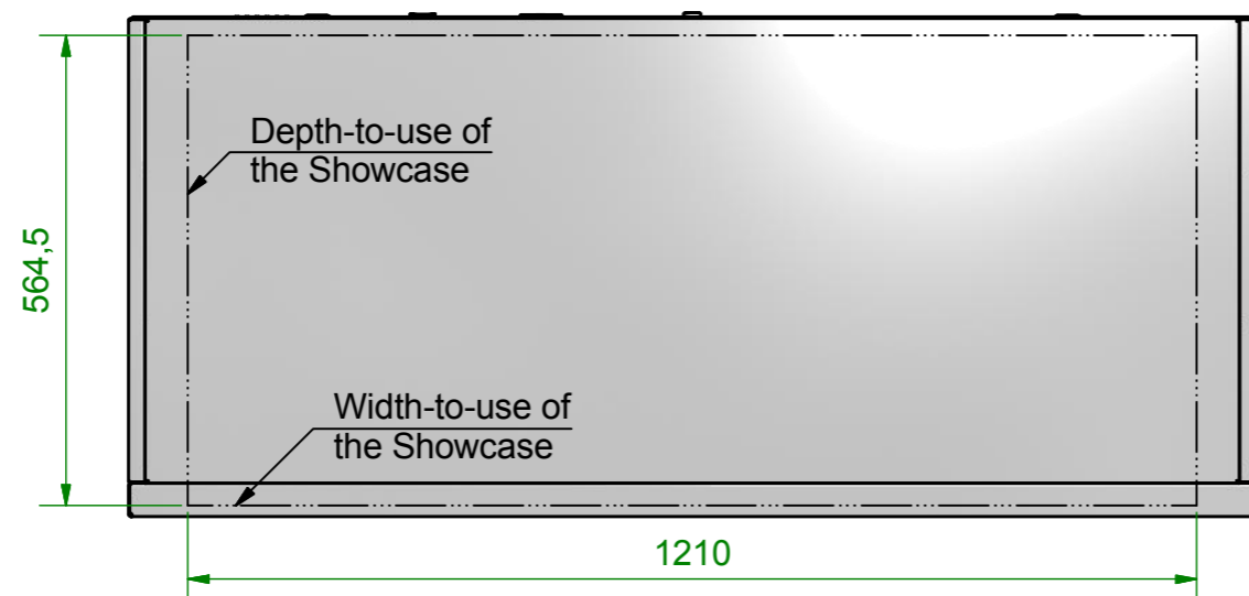
Top View 1:10
