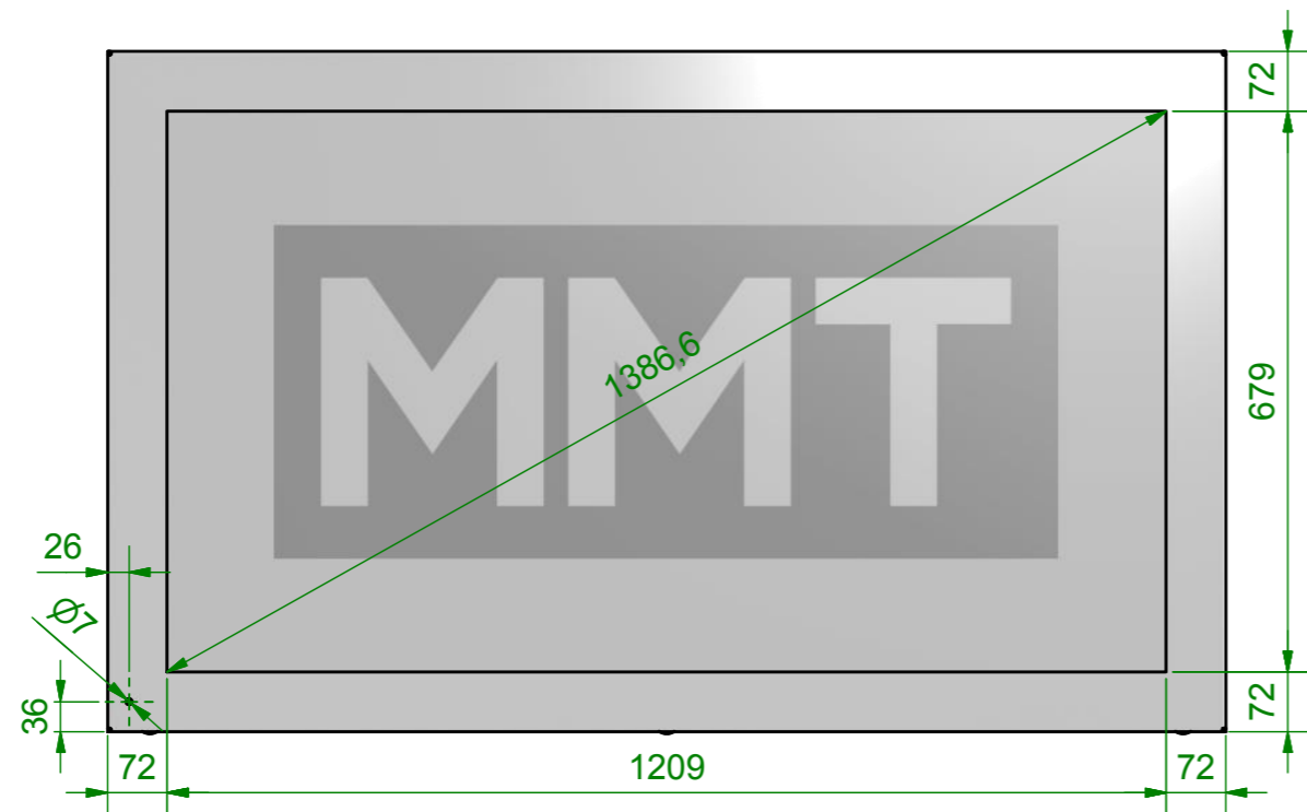
Front View 1:10
