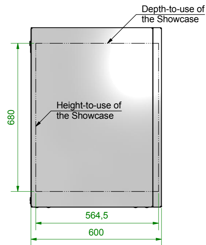
Lefthand View 1:10
