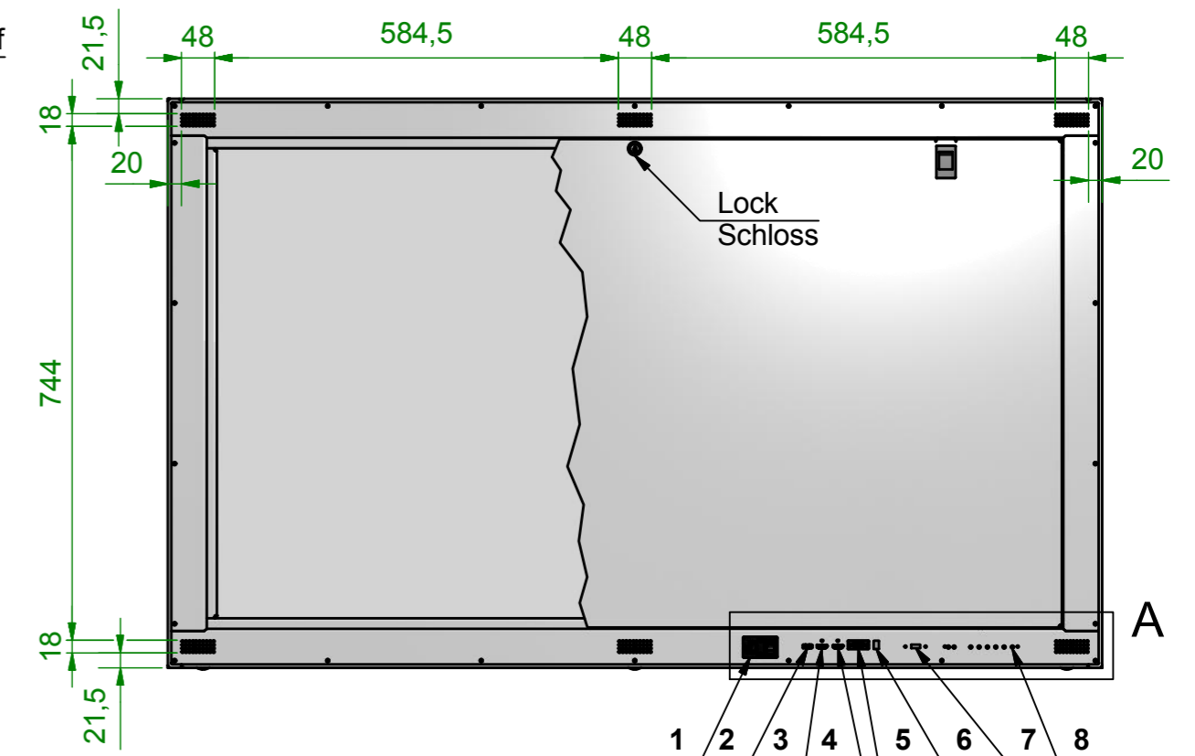
Back View 1:10
