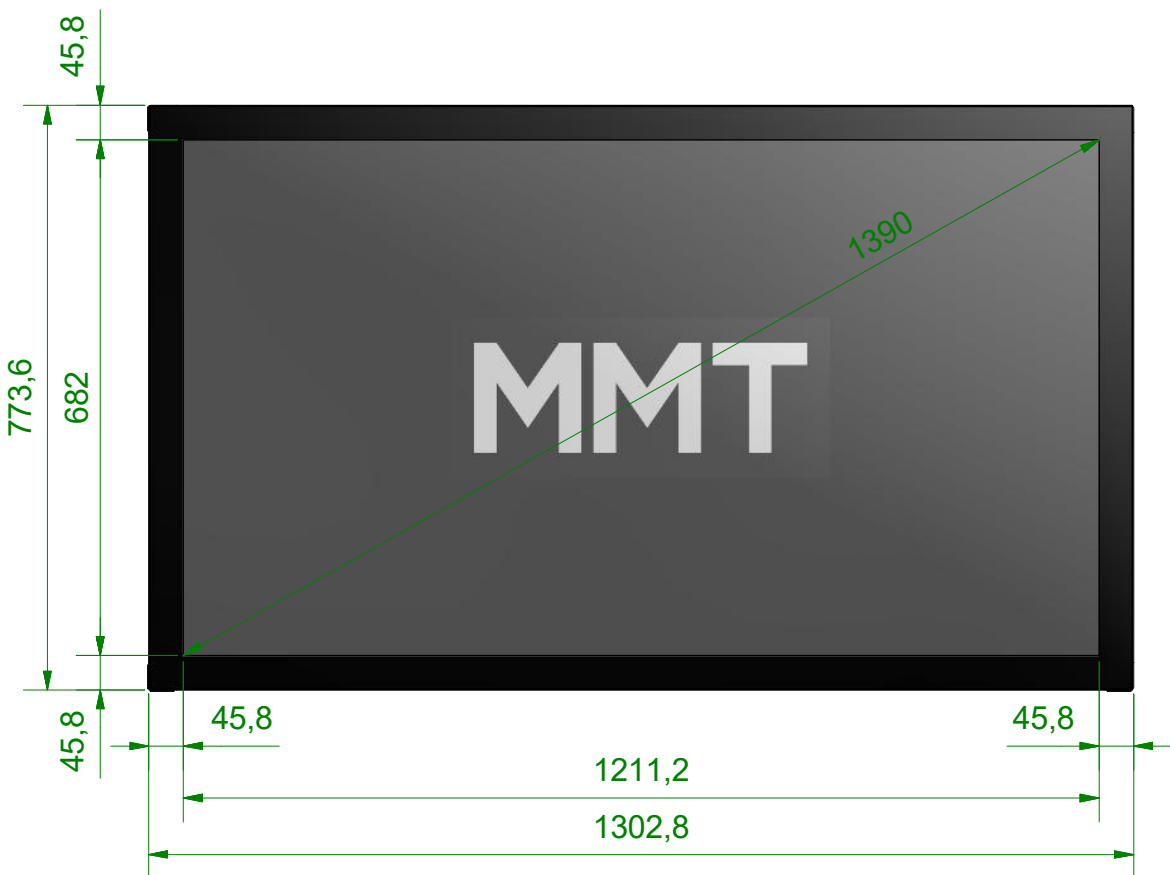
Top View 1 : 10
