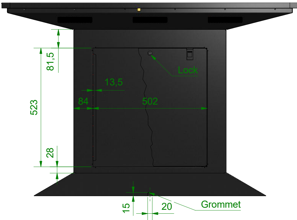
Back View 1 : 10
