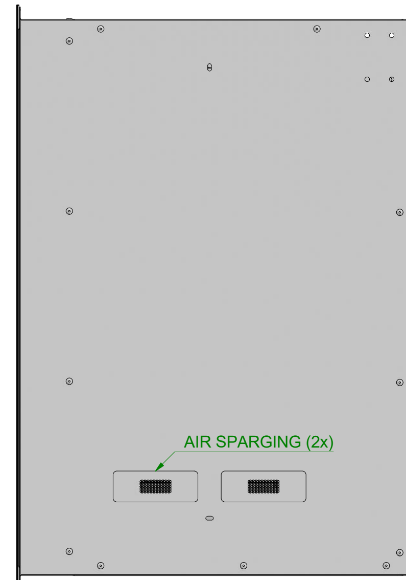
Righthand View 1:5
