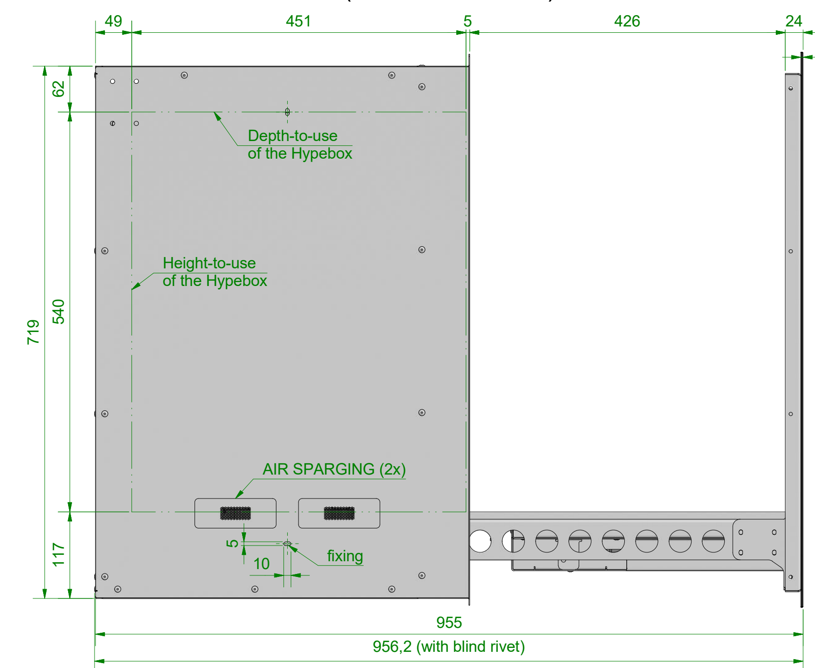
Lefthand View 1:5 (DRAWER OPEN)
