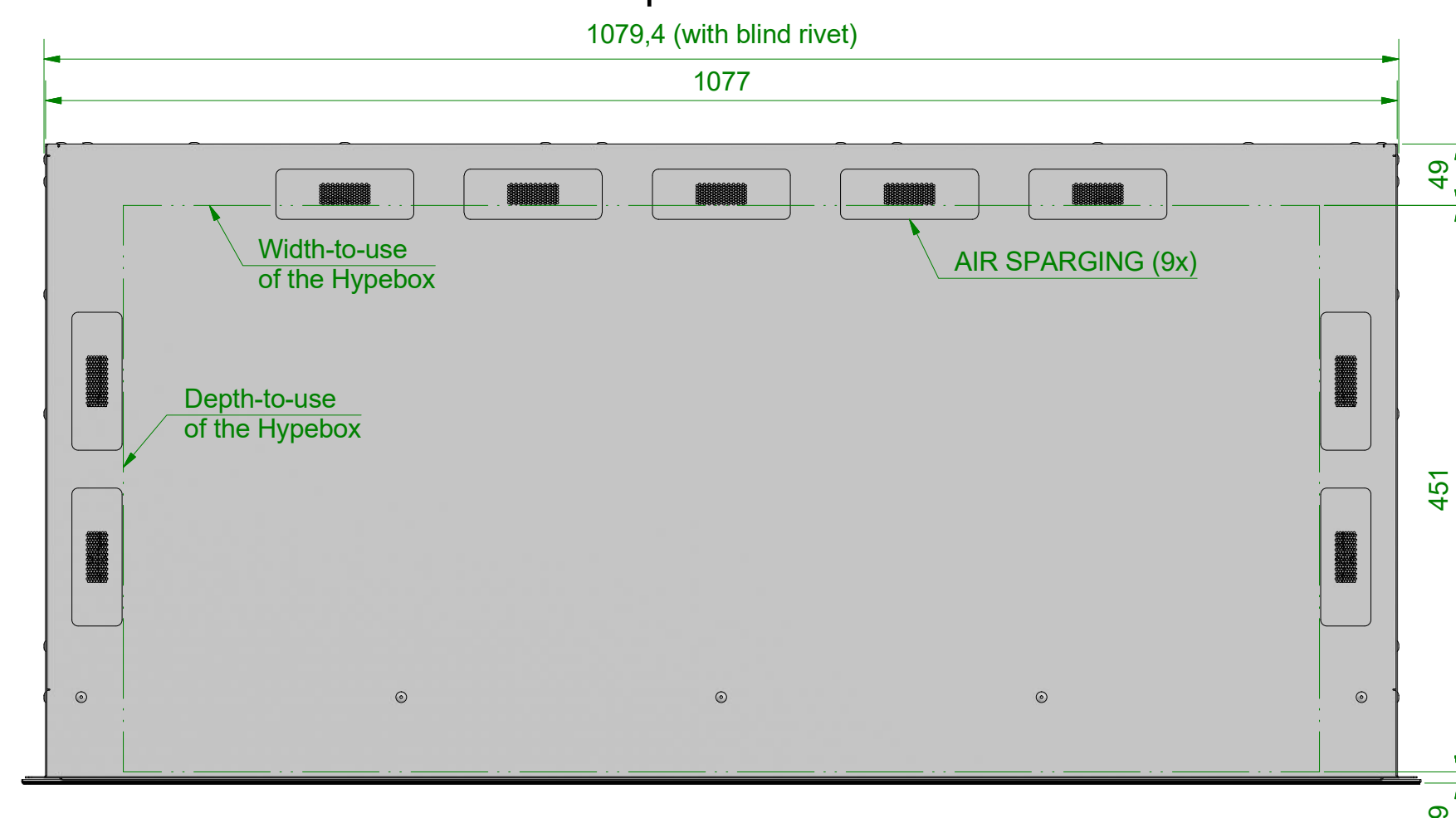
Top View 1:5
