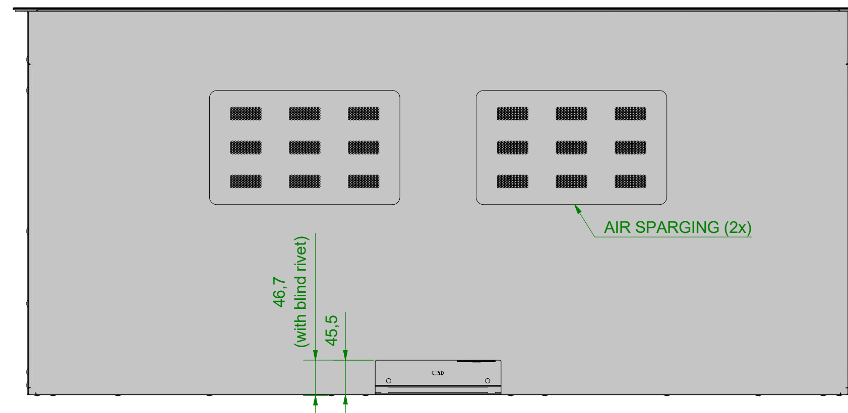
Bottom View 1:5
