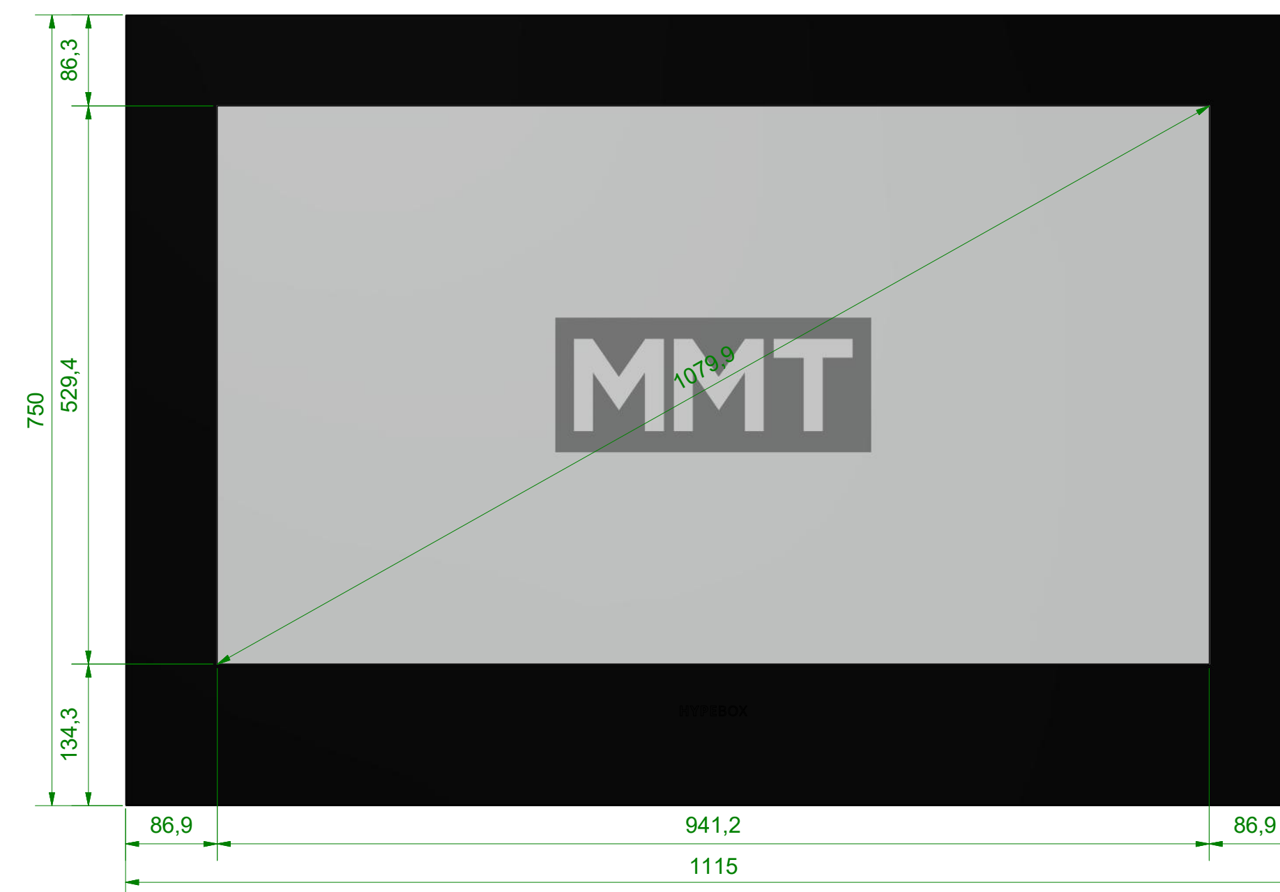
Front View 1:5
