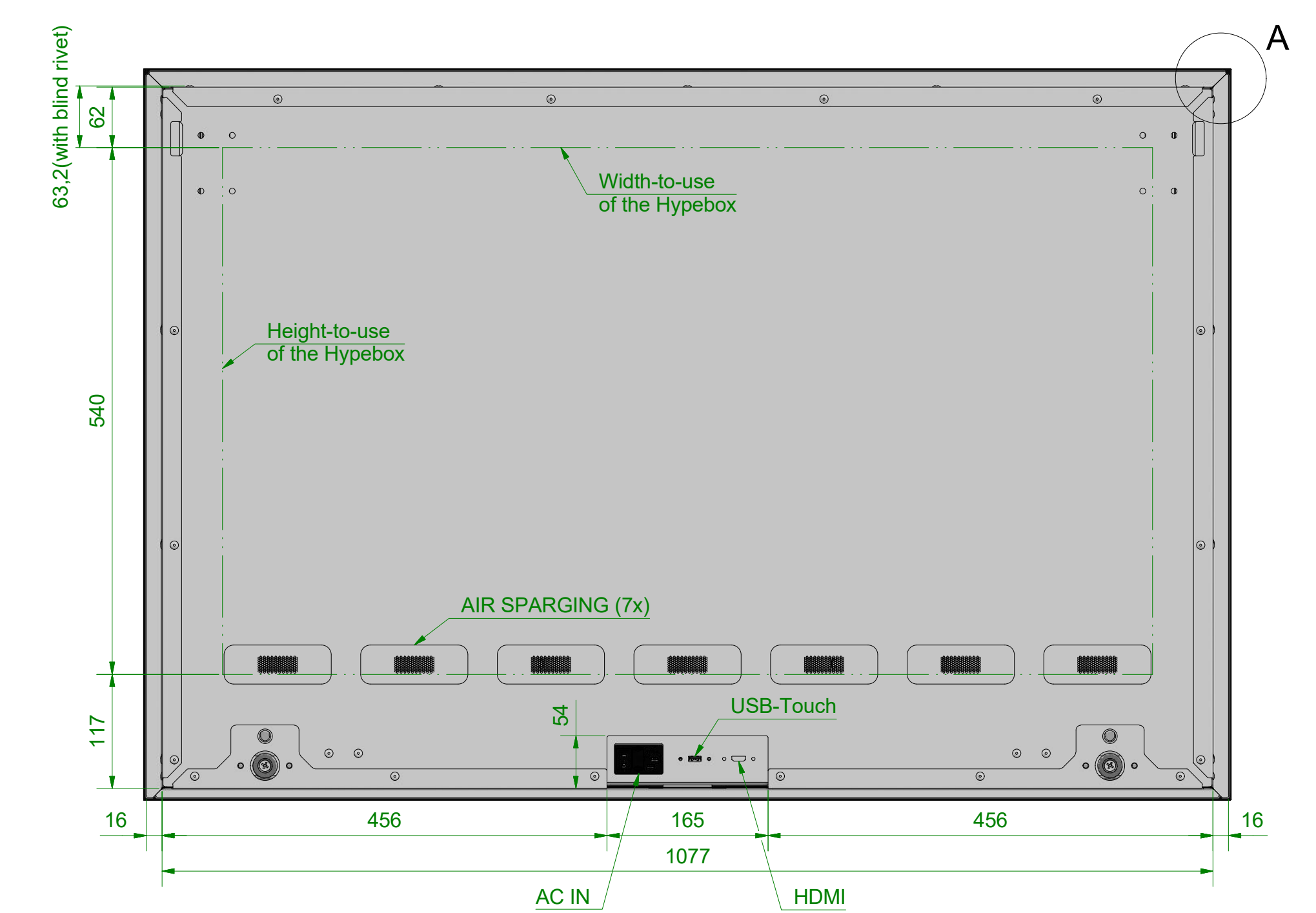
Back View 1:5
