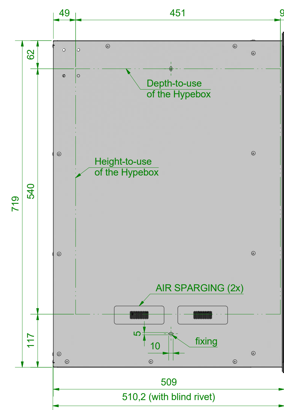
Lefthand View 1:5
