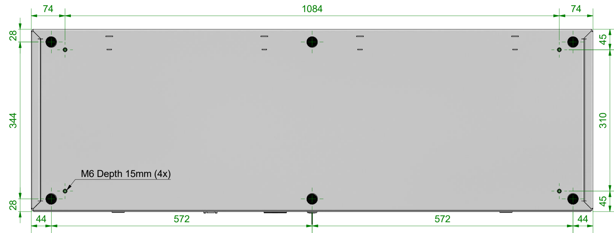
Bottom View 1:5
