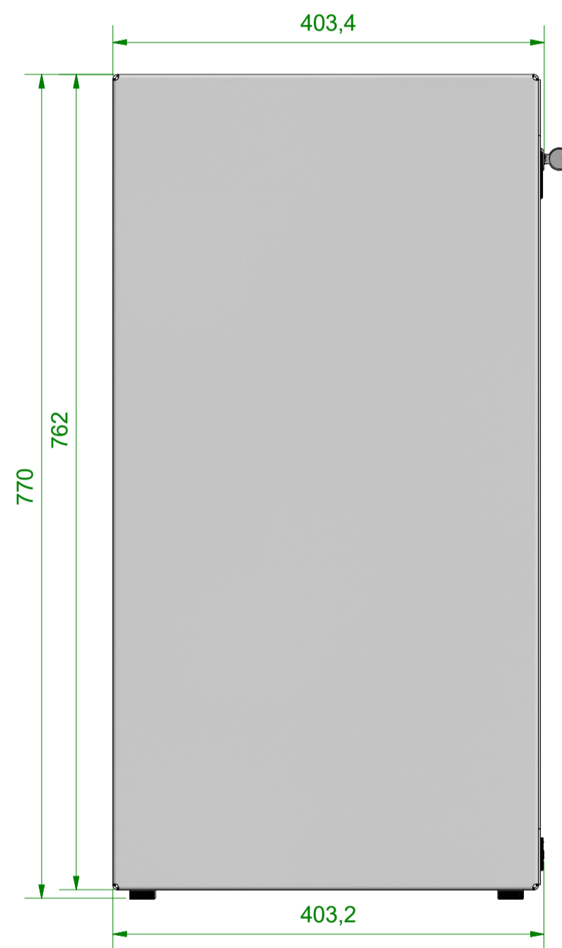
Righthand View 1:5
