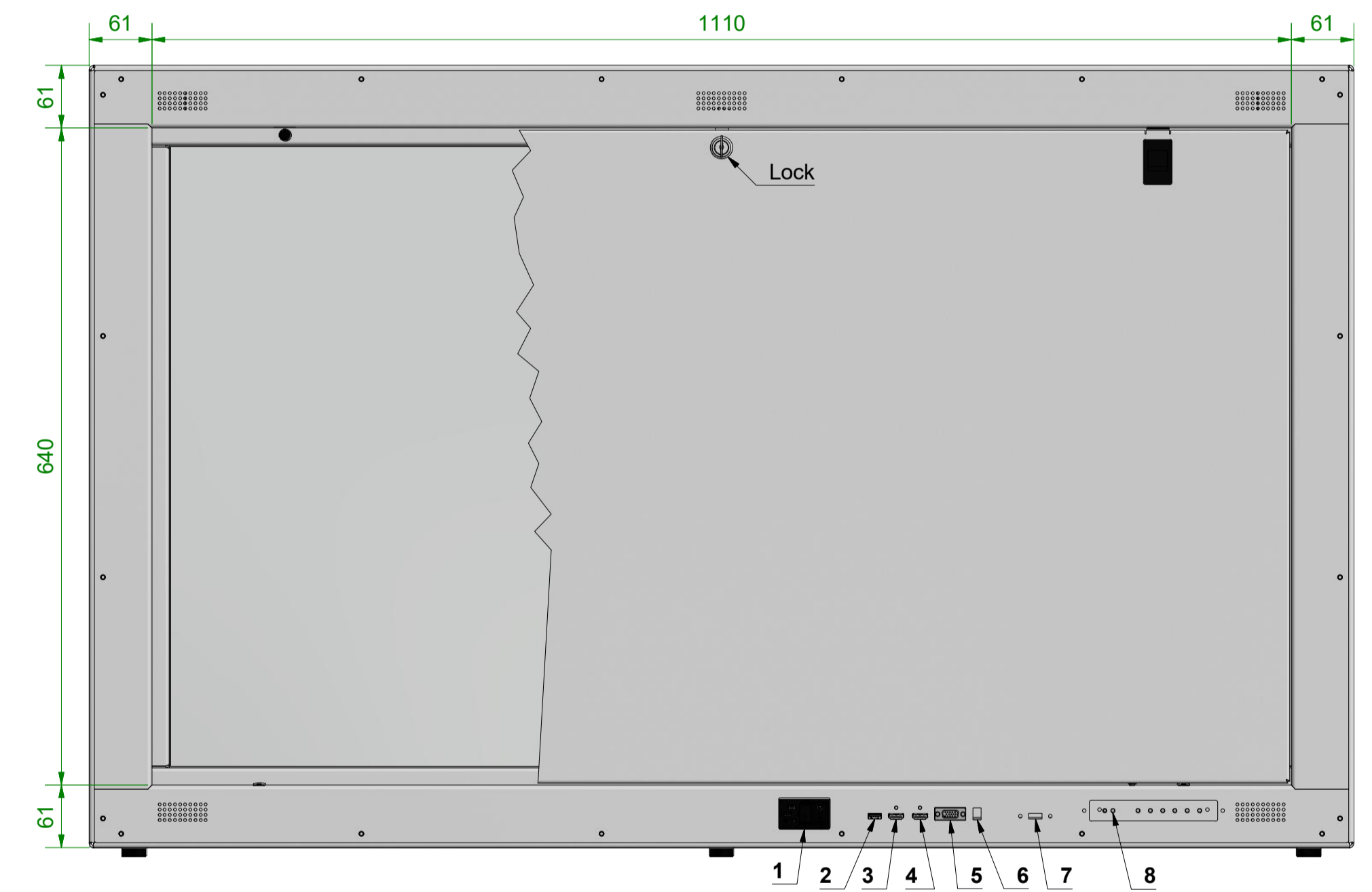
Back View 1:5
