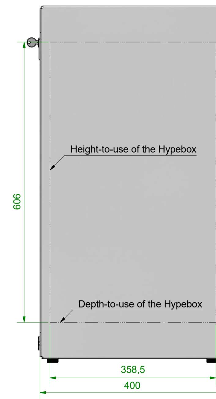
Lefthand View 1:5
