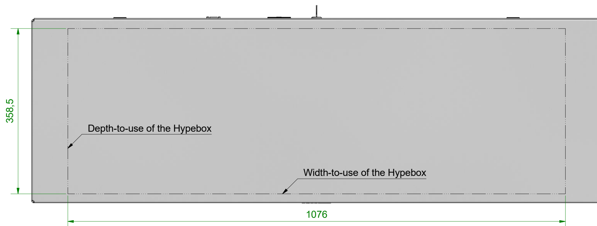
Top View 1:5
